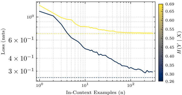
In-Context Learning Loss for Qwen-2.5 (3B)
